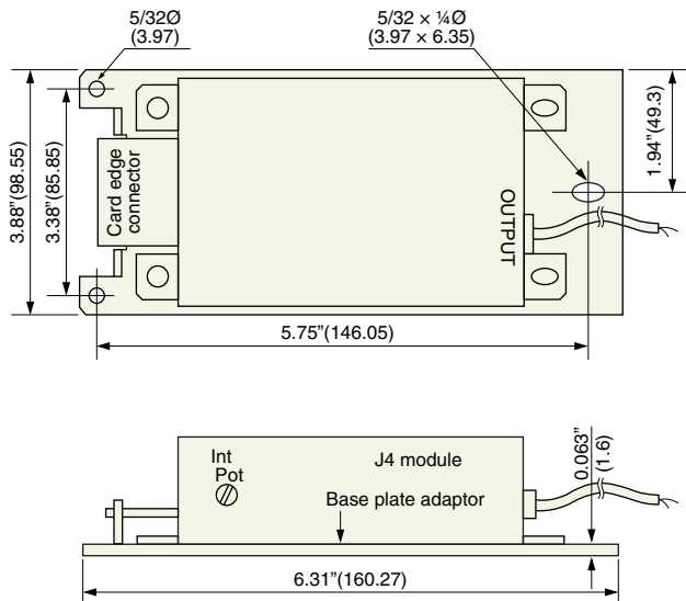
J4-LX
