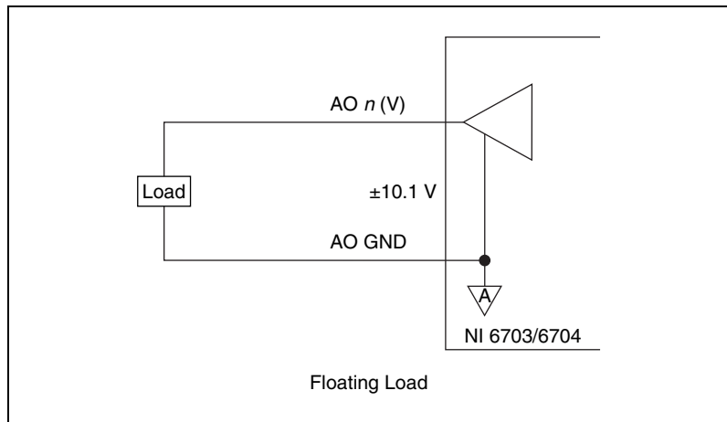
Figure 2-2. Voltage Output Connections
