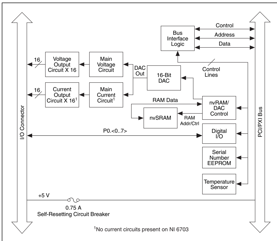
Figure 3-1. NI 6703/6704 Block Diagram
